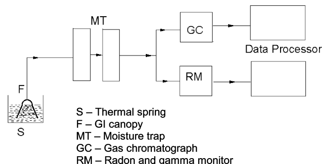
Figure 1. Block diagram of integrated experimental arrangement.
